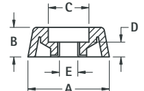
FIG. 3 Mold-In Washer
