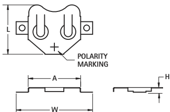
FIG. 1 - Compact
