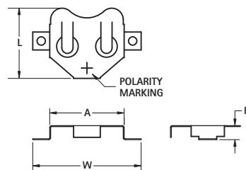
FIG. 2 - Low Profile
