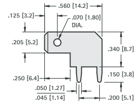
.205 (5.2) TAB
