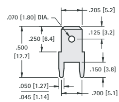
.205 (5.2) TAB
