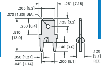
.205 (5.2) TAB
